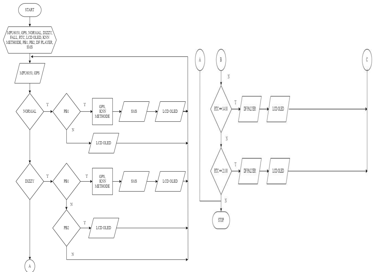
FIG 5. Flowchart of Fall Detection Tool
