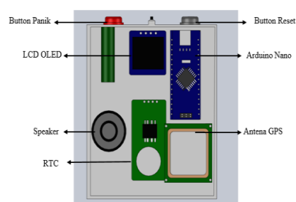
FIG 3. Tool Prototype Design
