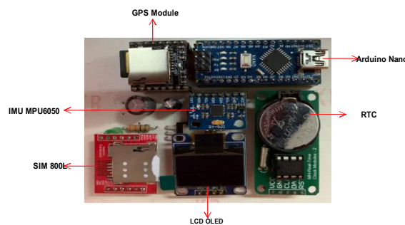
FIG 2. Electronic circuit of a fall detection device
