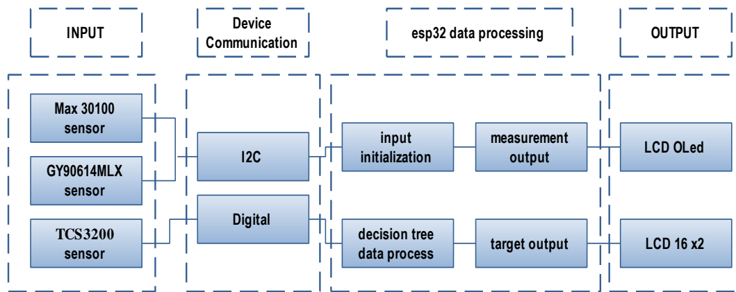
FIG 1. Block Diagram System for measuring basic vital signs and early detection of dehydration in the human body
